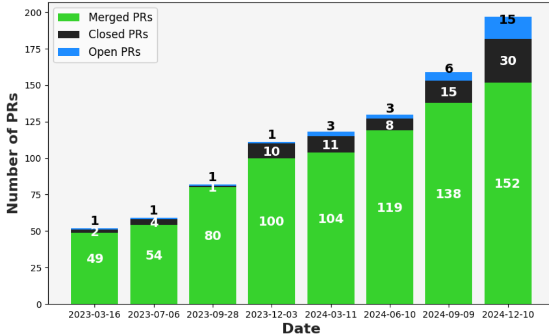
PR Statistics for Dasharo/edk2 fork
