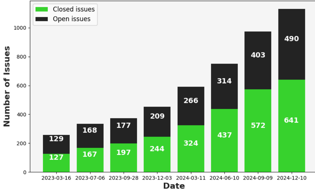
Dasharo Issues Statistics
